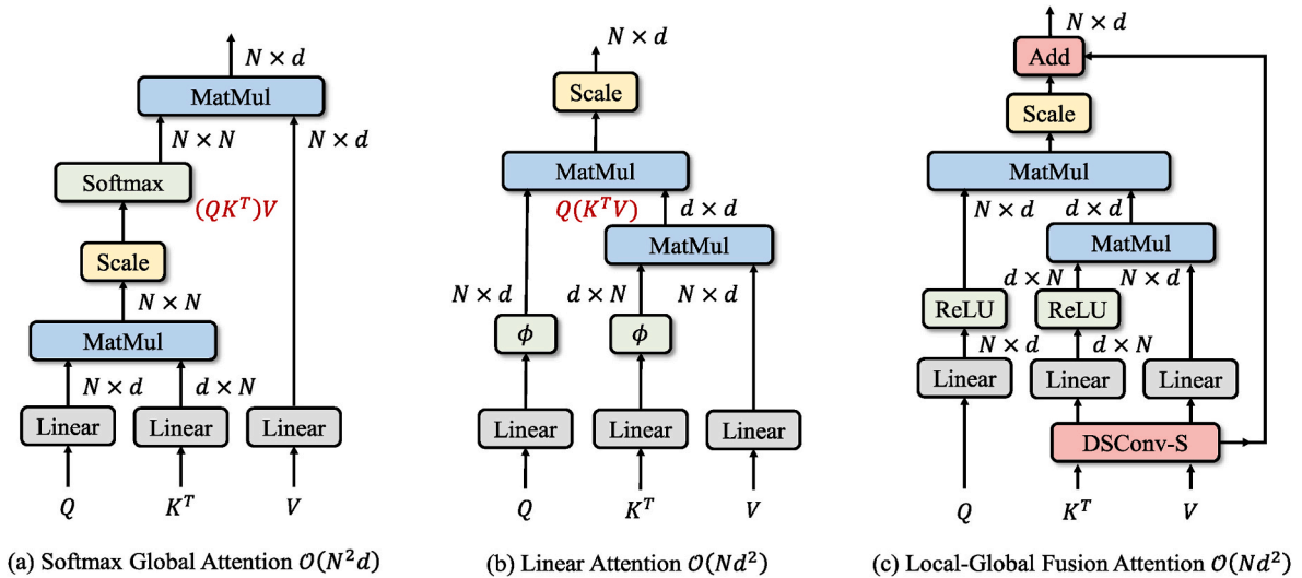
Fig. 6. Difference between (a) traditional Softmax attention mechanism, (b) traditional Linear Attention mechanism, and (3) the proposed Local-Global Fusion attention module.
