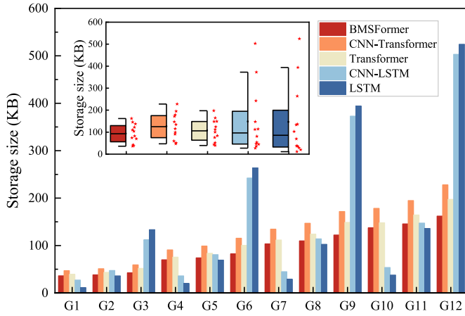
Fig. 8. Storage size of five models across G1-G12 hyperparameter combinations: (a) Bar chart comparing storage sizes for each group; (b) Box plot showing overall distribution.
