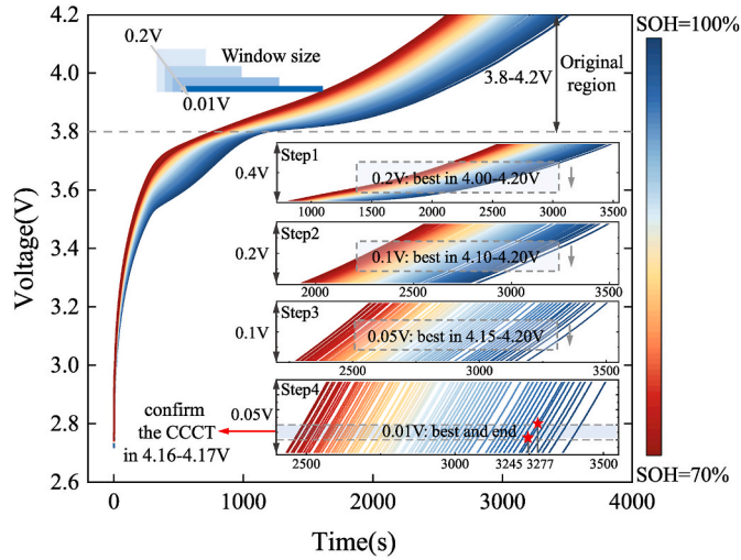
Fig. 3. The extraction procedures of the selected HI in the selected charge segment.
