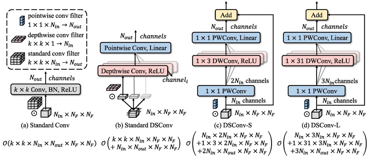
Fig. 5. The fundamental structure of: (a) Standard convolution; (b) Standard Depthwise separable convolution; (c) DSConv-S module; (d) DSConv-L module.
