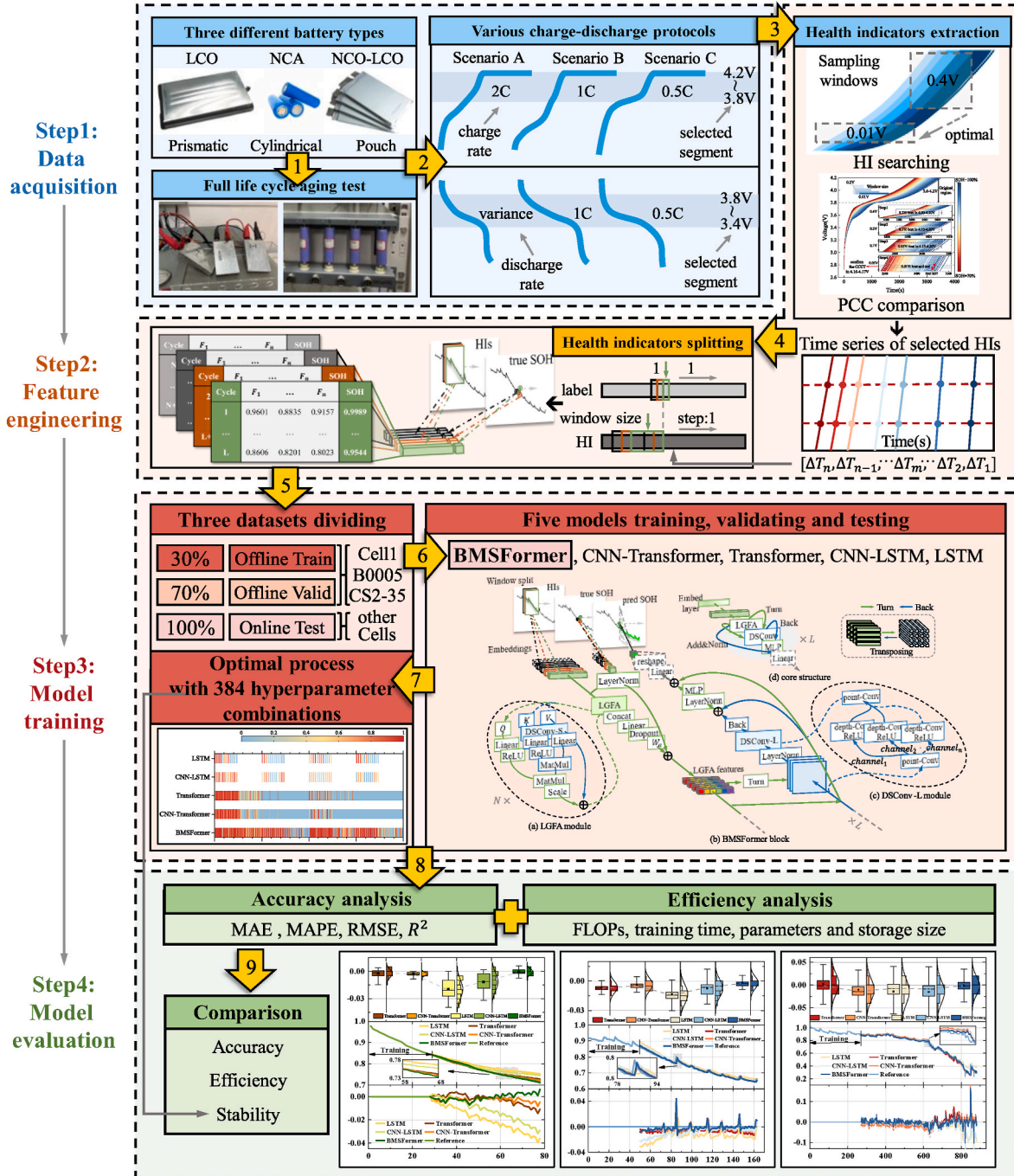
Fig. 1. Flowchart of developed SOH estimation approach.
