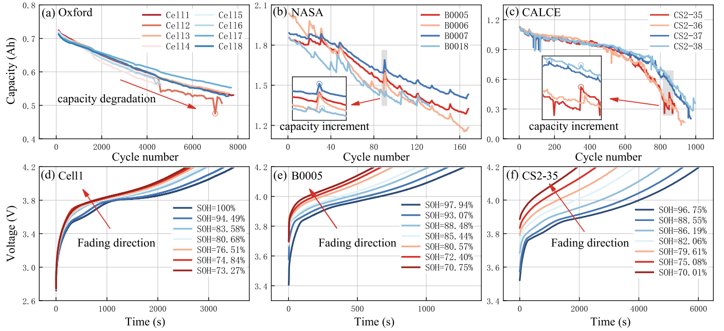
Fig. 2. Three different kinds of battery datasets: (a)–(c) capacity degradation and temporary increment curves of the Oxford, NASA and CALCE cells, respectively. (d)–(f) constant current charge voltage curves of Oxford Cell1, NASA B0005 and CALCE CS2-35, respectively.
