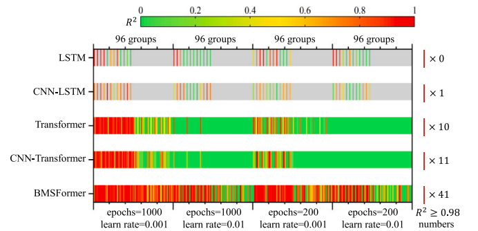
Fig. 9. The whole validating results when using different models and hyperparameter combinations.
