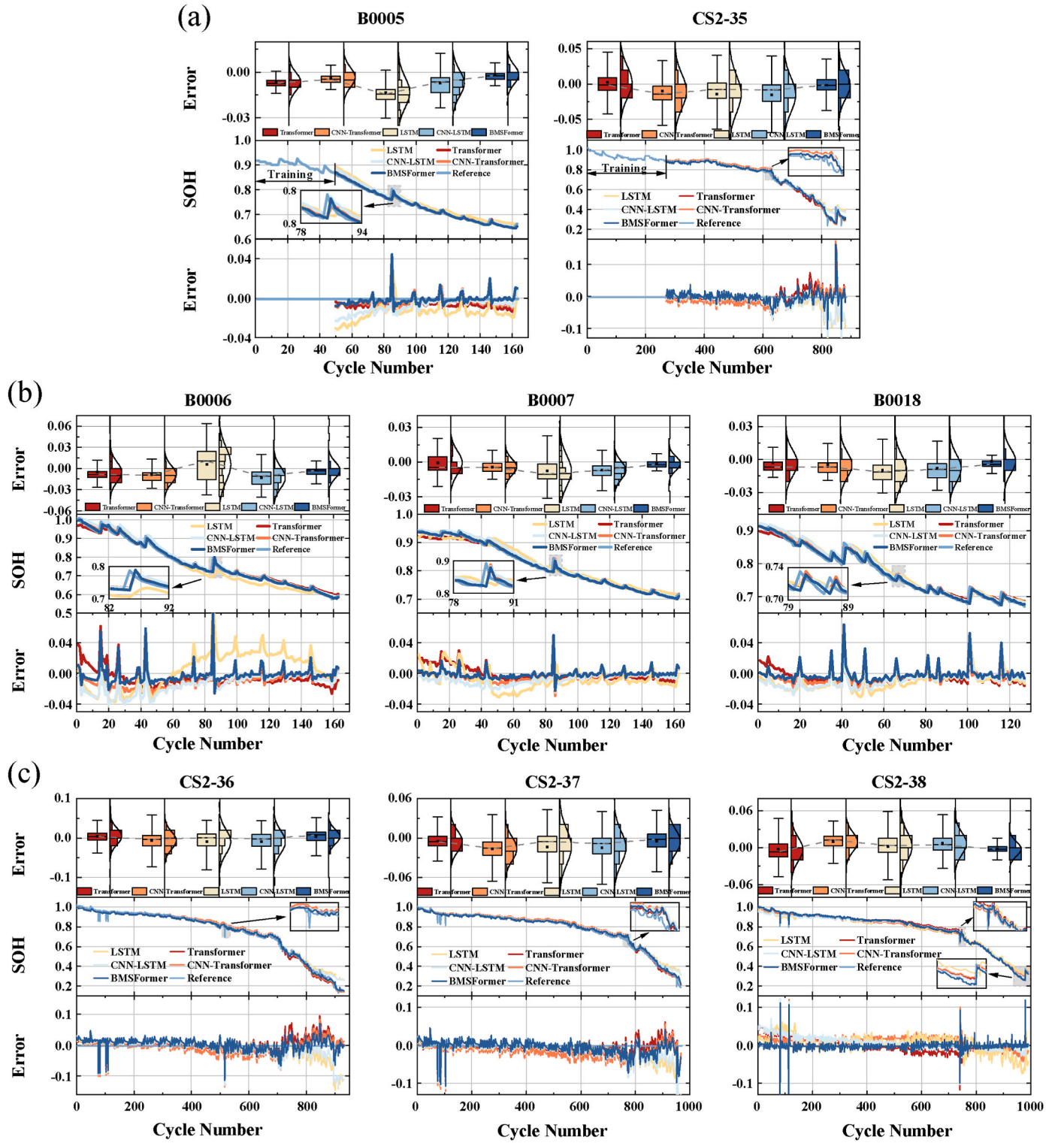
Fig. 10. (a) The validation results of five models on B0005 and CS2-35. (b) The test results using five weighted models trained on B0005. (c) The test results using five weighted models trained on CS2-35.
