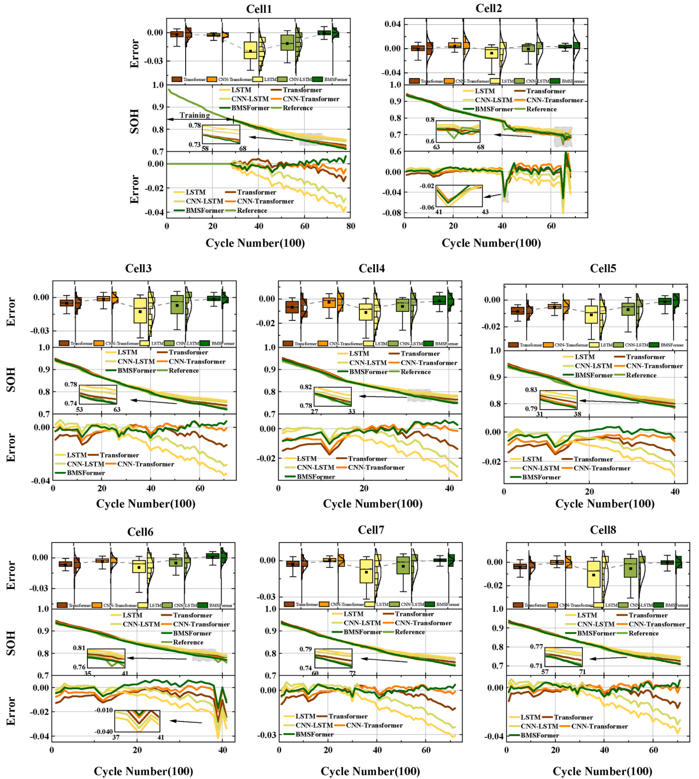
Fig. 7. The experimental results of different models on the Oxford dataset.
