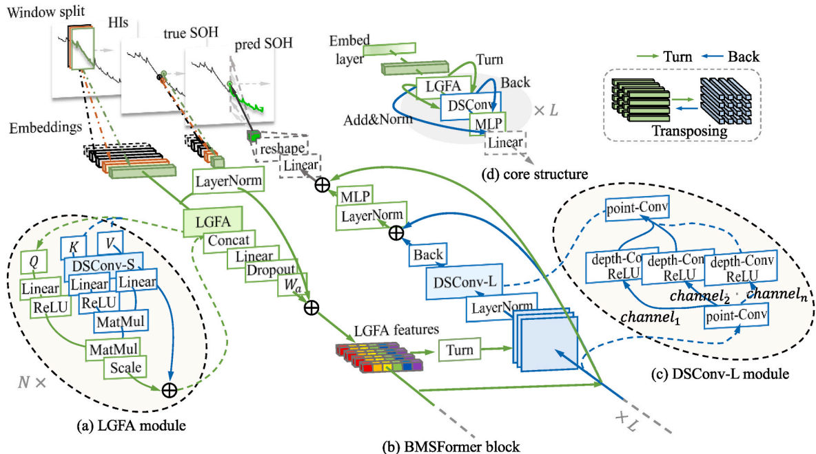
Fig. 4. Framework of BMSFormer. (a) LGFA module, (b) BMSFormer block, (c) DSConv-L module, (d) BMSFormer core structure.
